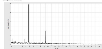
PT501 Envelope Analysis
